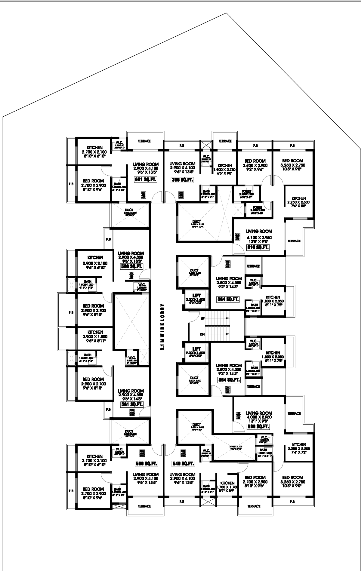
← 15 M . WIDE ROAD → TYPICAL FLOOR PLAN ( 2ND, 4TH , & 6TH )
